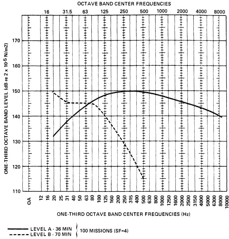
Figure 7. Acoustic Test Environment for Wing Leading Edge
