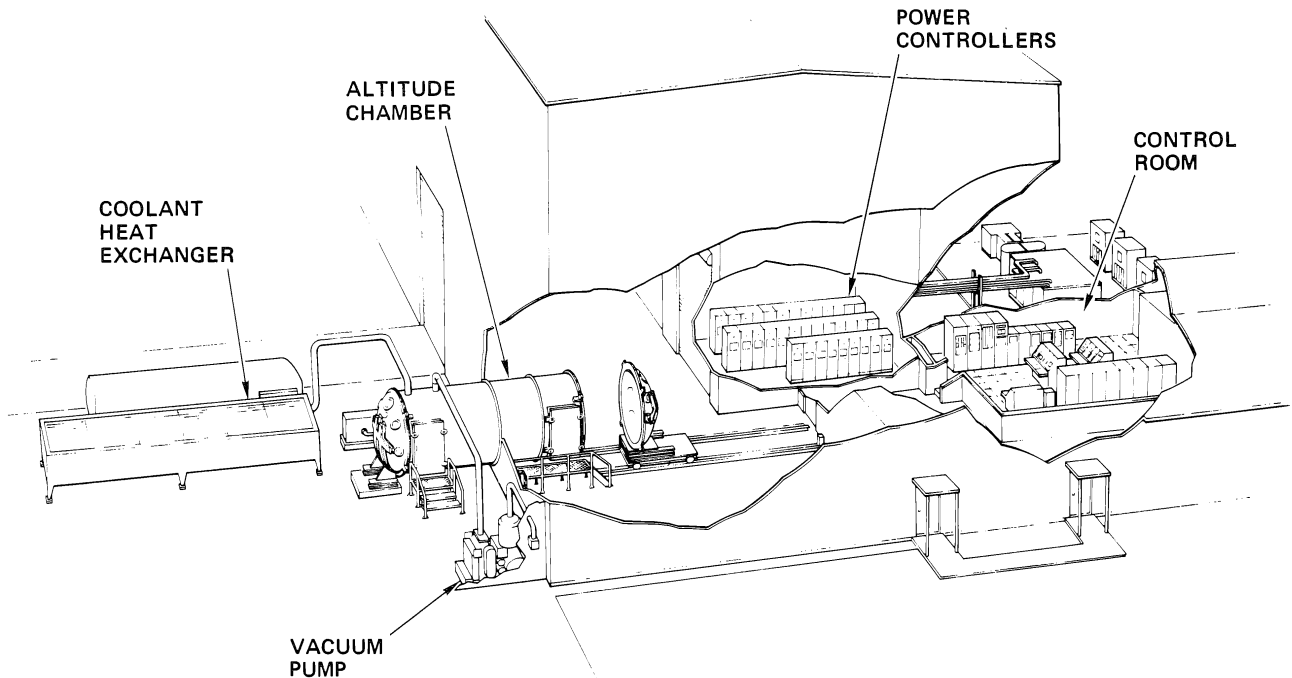
Figure 13. Radiant Heating Test Facility
