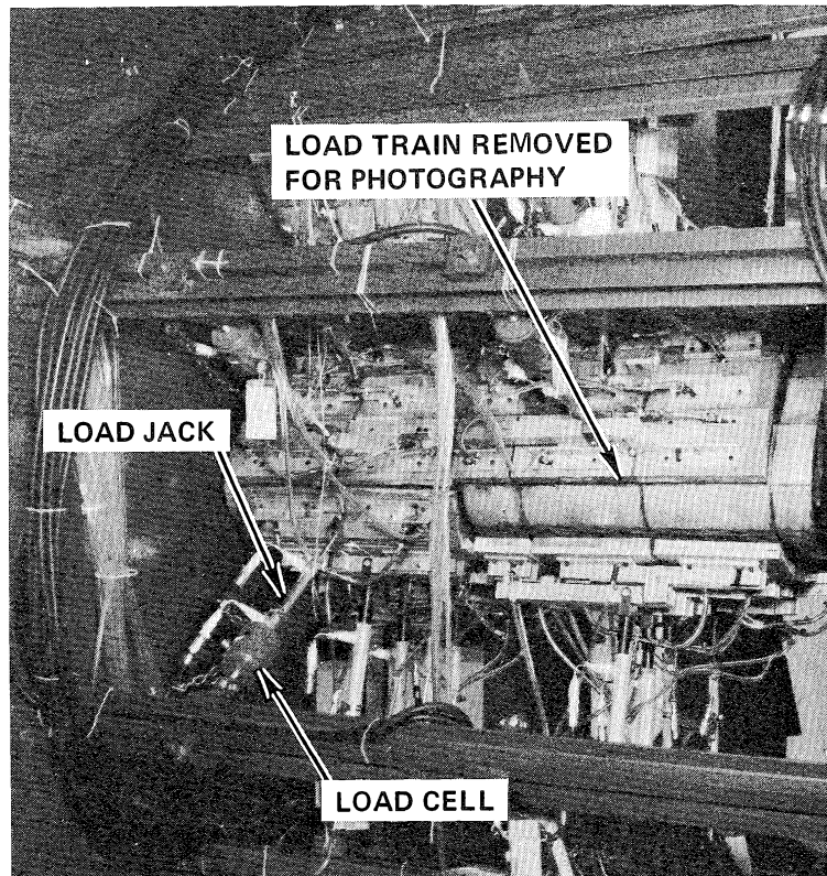
Figure 10. Wing Leading Edge Airloads Test Setup
