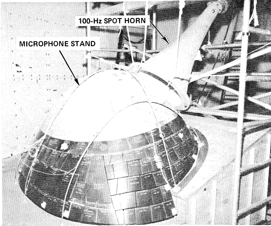
Figure 5. Nose Cap Acoustic Test Setup
