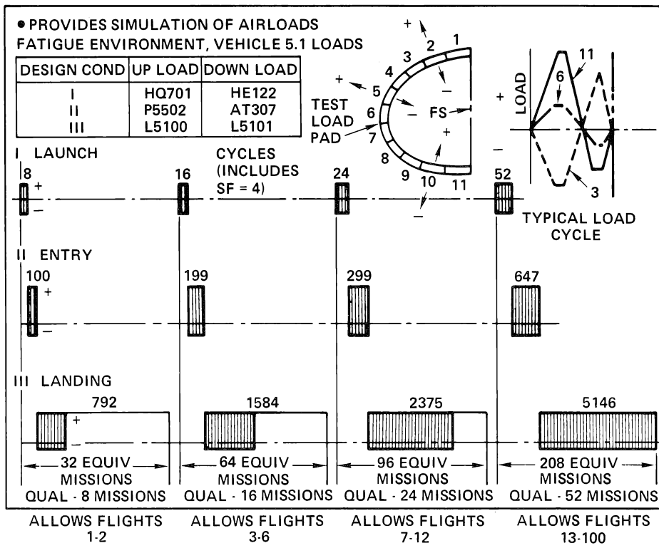
Figure 12. Wing Leading Edge Airloads Spectrum
