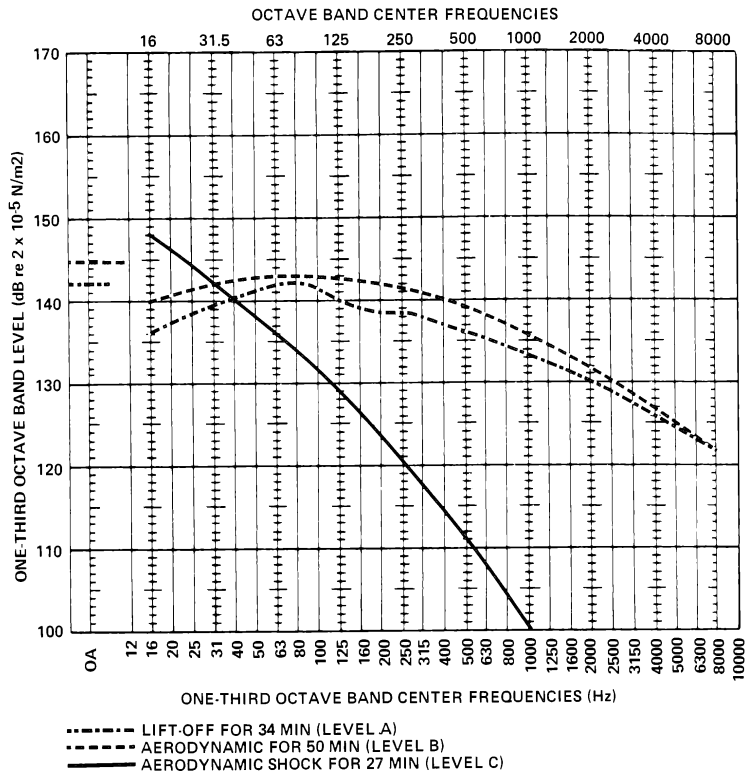
Figure 6. Acoustic Test Environment for Nose Cap
