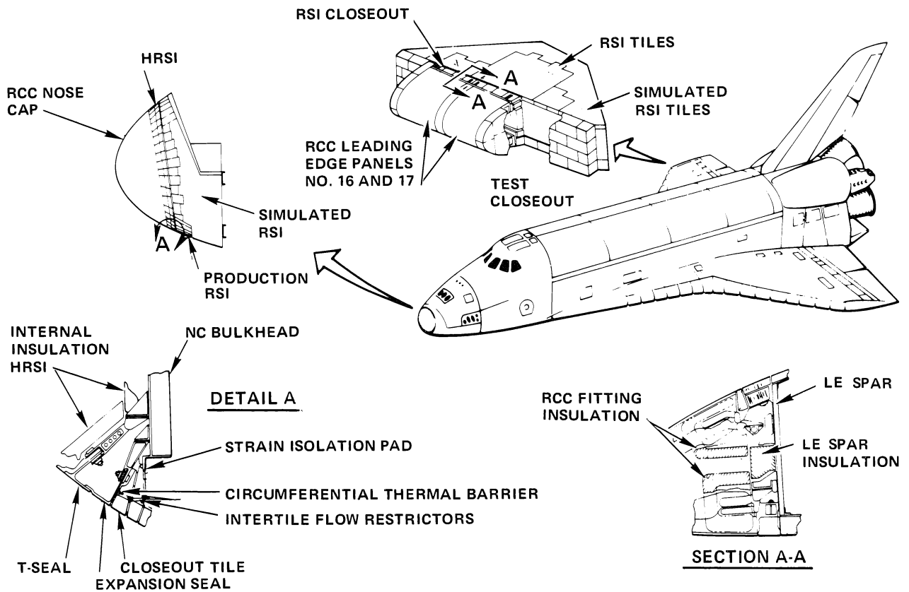
Figure 2. Nose Cap and Wing Leading Edge Test Articles
