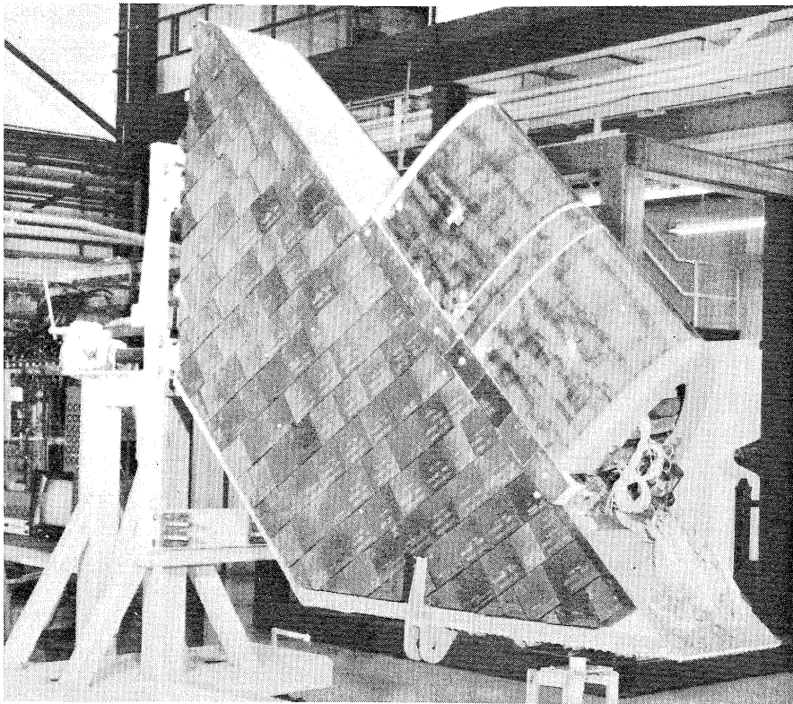
Figure 4. Wing Leading Edge Test Article
