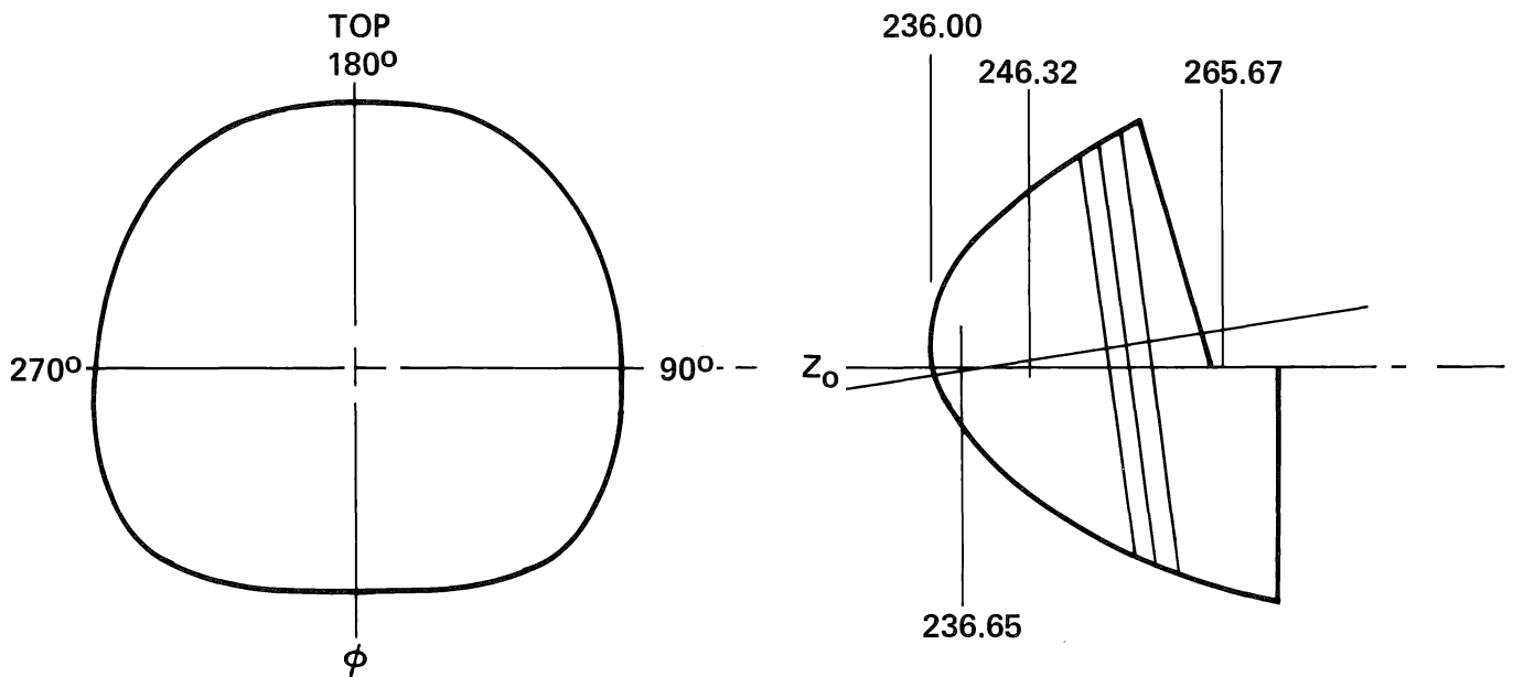
Figure 11. Nose Cap Design Limit Loads
