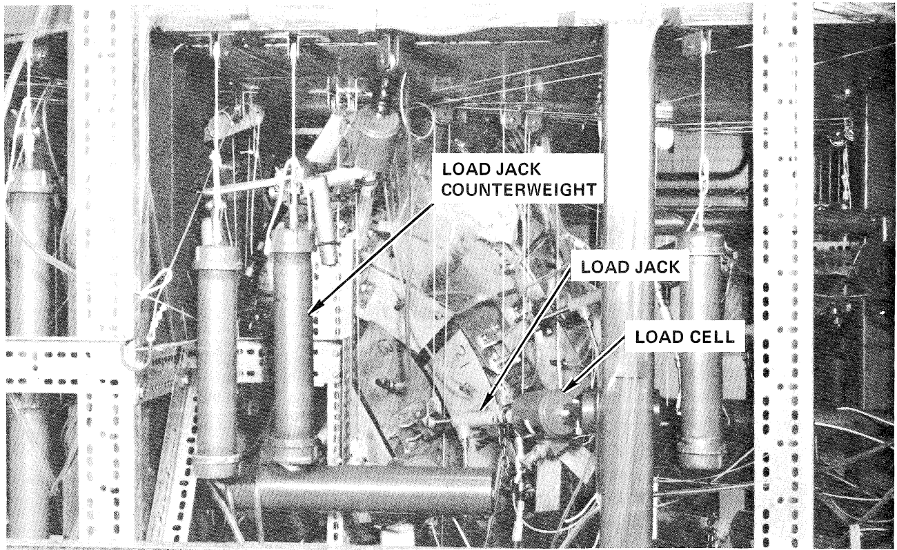
Figure 9. Nose Cap Airloads Test Setup
