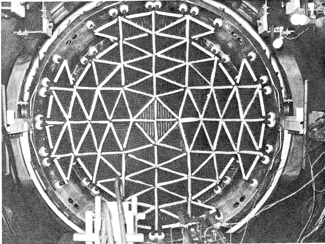
Figure 14. Nose Cap Heater
