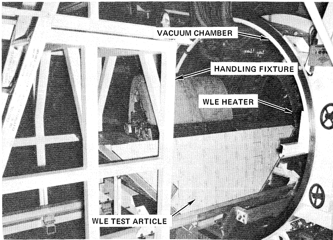
Figure 16. Wing Leading Edge Test Setup
