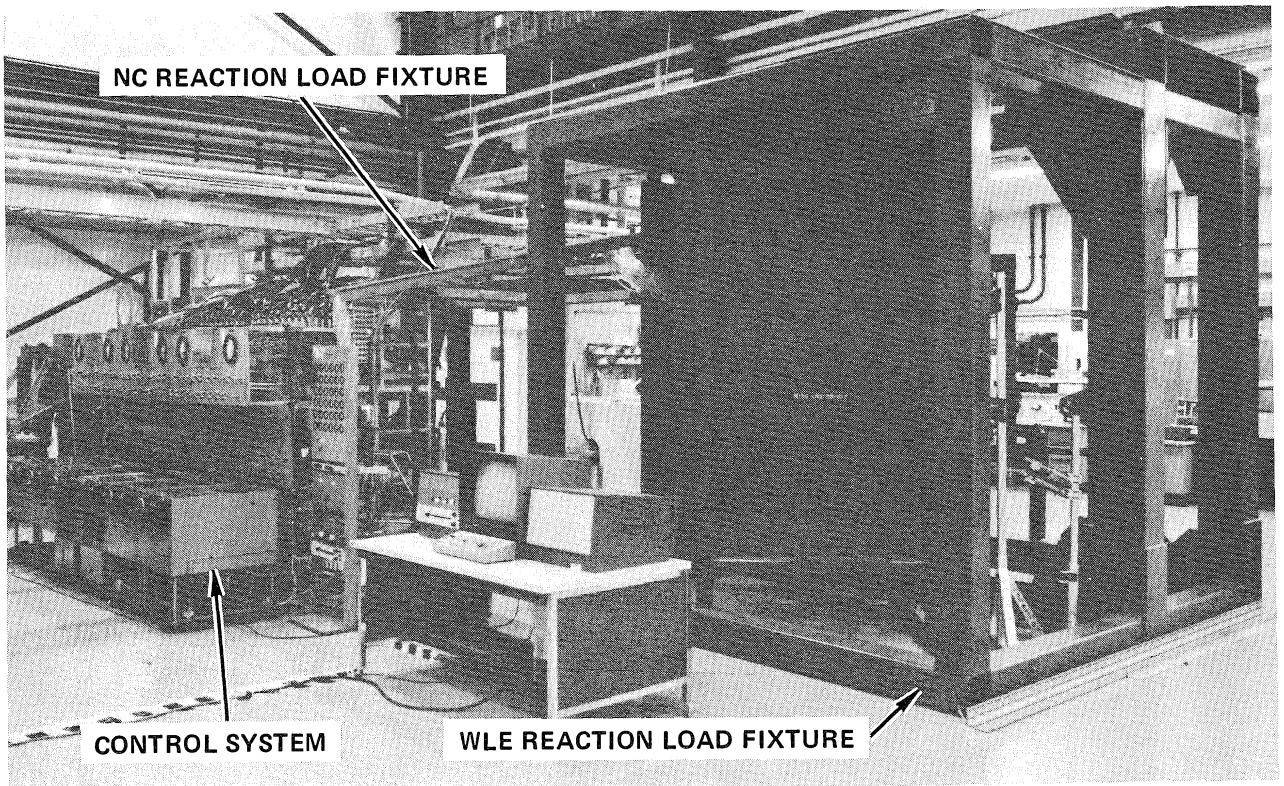
Figure 8. Airloads Test Setup
