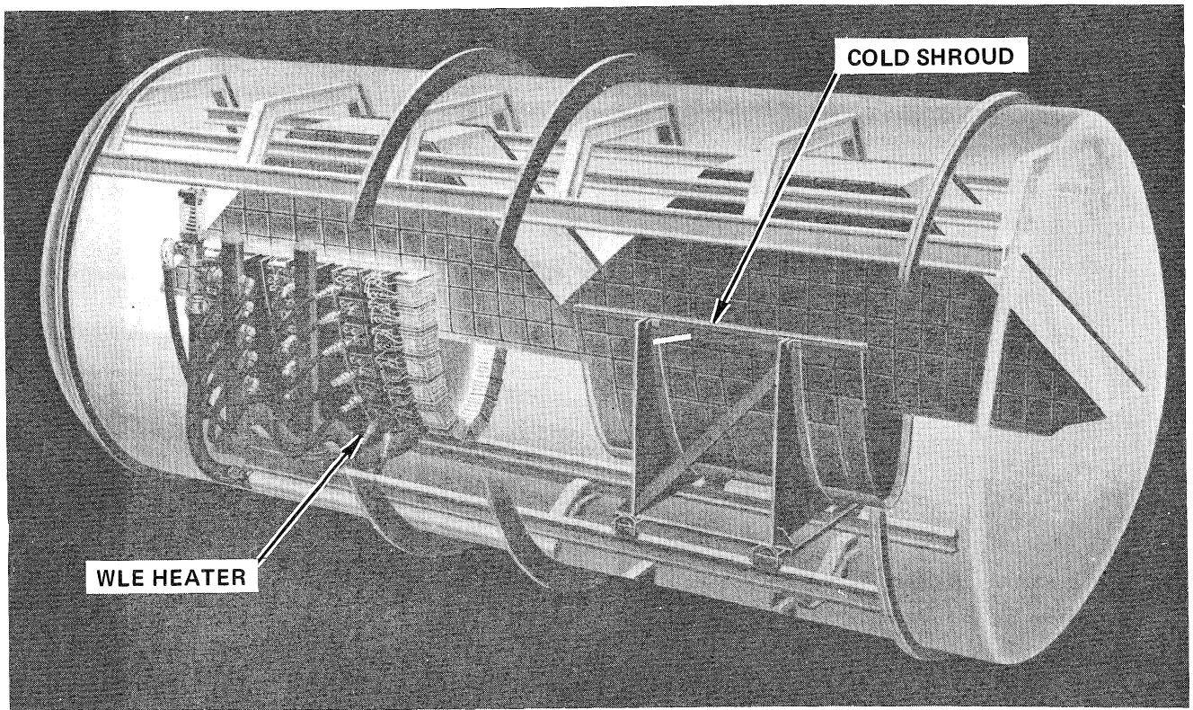
Figure 15. Artist's Concept of Wing Leading Edge Test System (Test Article Shown in Both the High- and Low-Temperature Positions)
