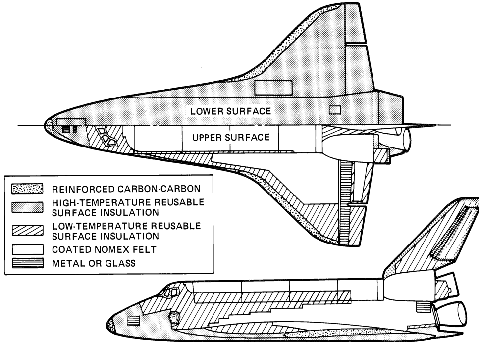
Figure 1. Orbiter Thermal Protection System
