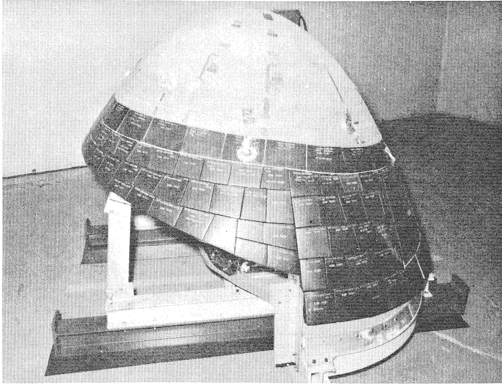
Figure 3. Nose Cap Test Article
